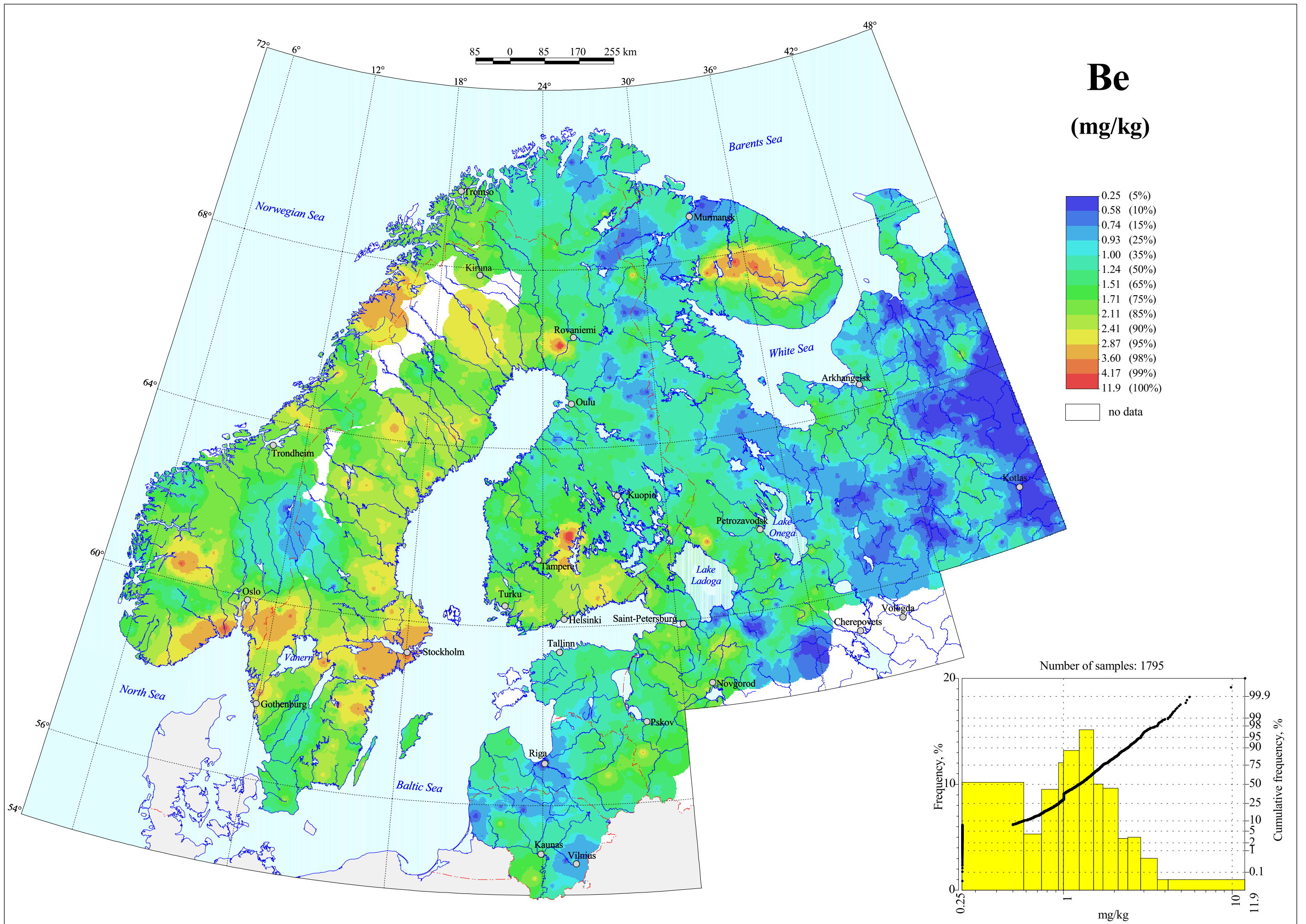
Beryllium in C-horizon, Grain Size <math>< 2\text{ mm}</math>, Total Content
