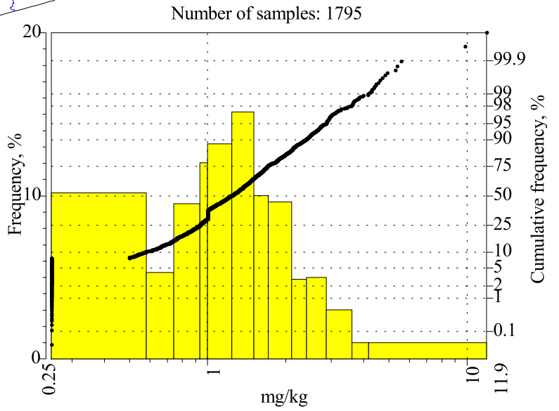
Beryllium in C-horizon, Grain Size <math>< 2\text{ mm}</math>, Total Content
